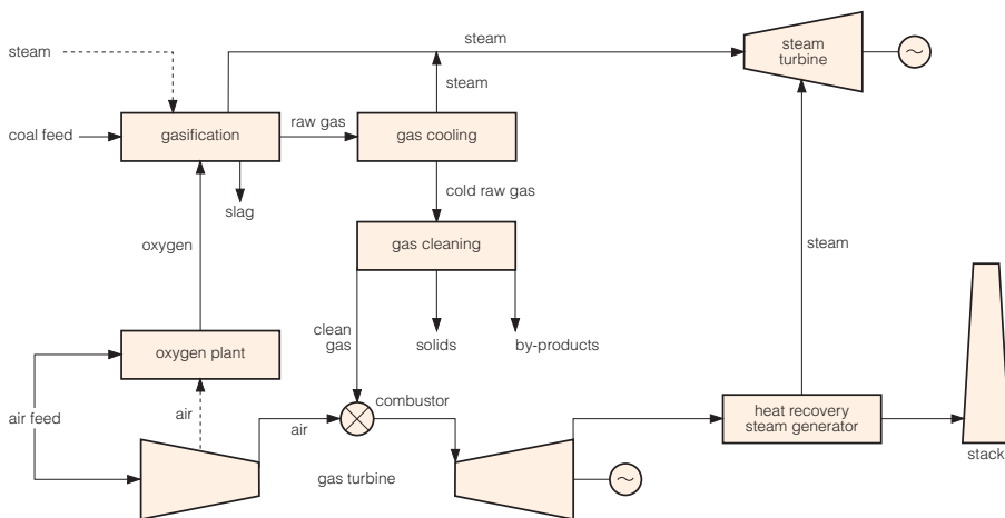
Integrated gasification combined cycle without CO 2 capture – major component systems
